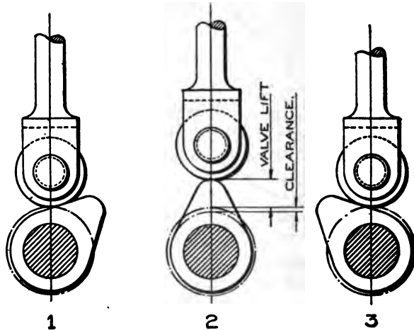
FIG. 212.—The Successive Positions of a Valve-lifting Cam (after Faurote).
